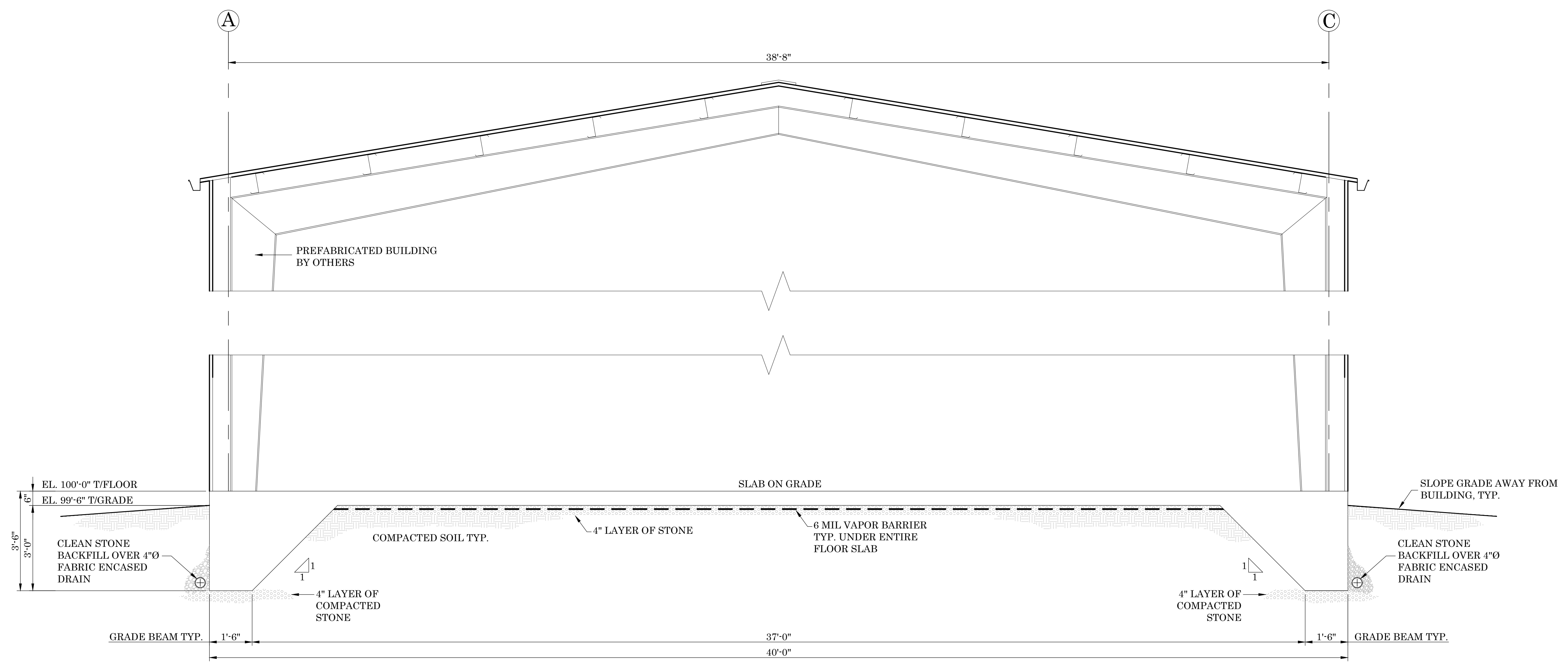
SECTION 1 - BUILDING THROUGH GRADE BEAMS
