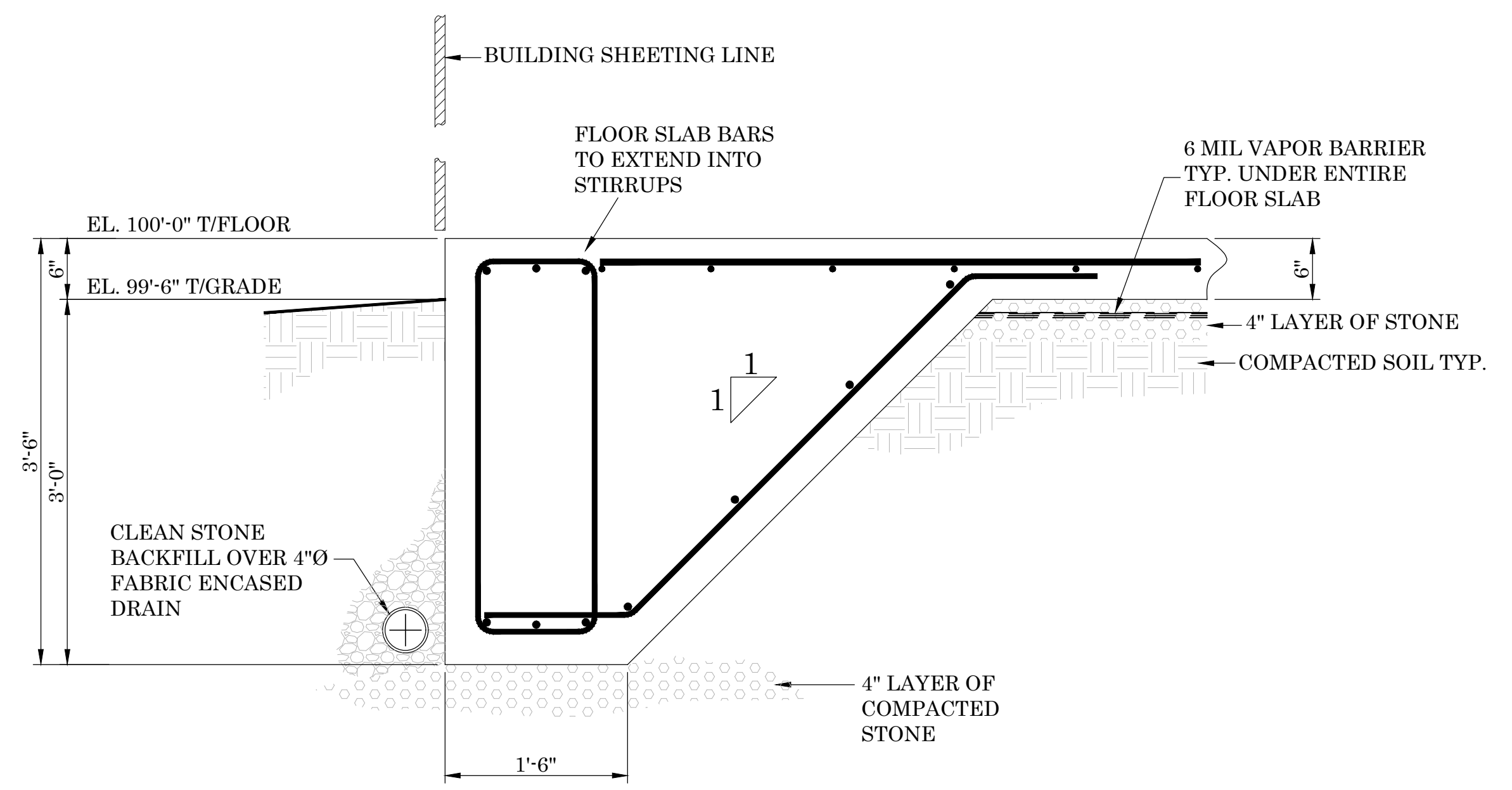
SECTION 2 - TYPICAL GRADE BEAM
